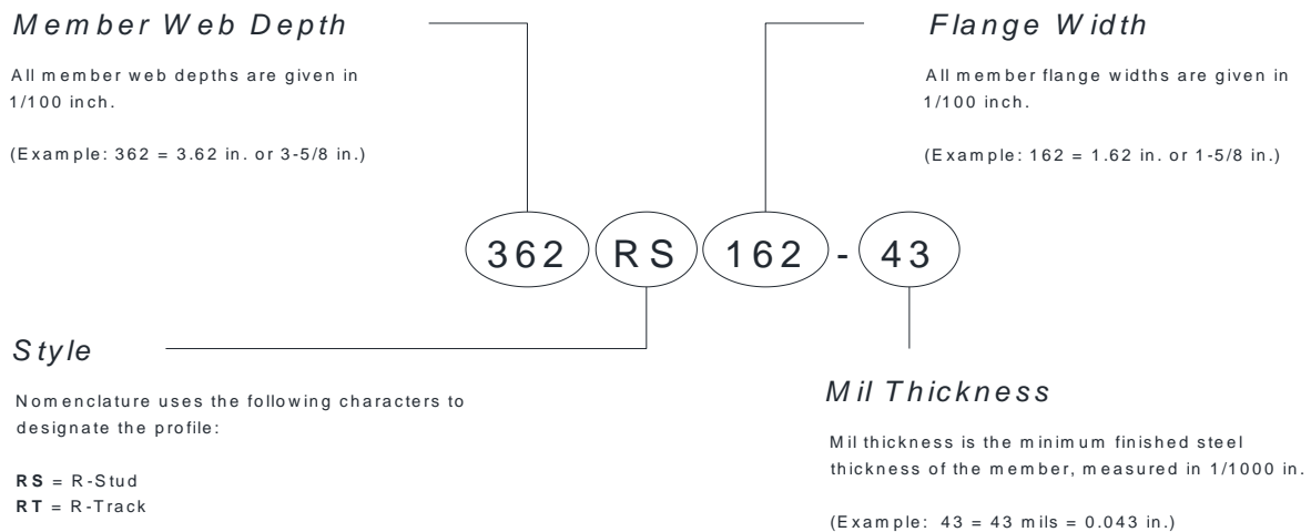
Figure 3. Stud and track designation nomenclature.
