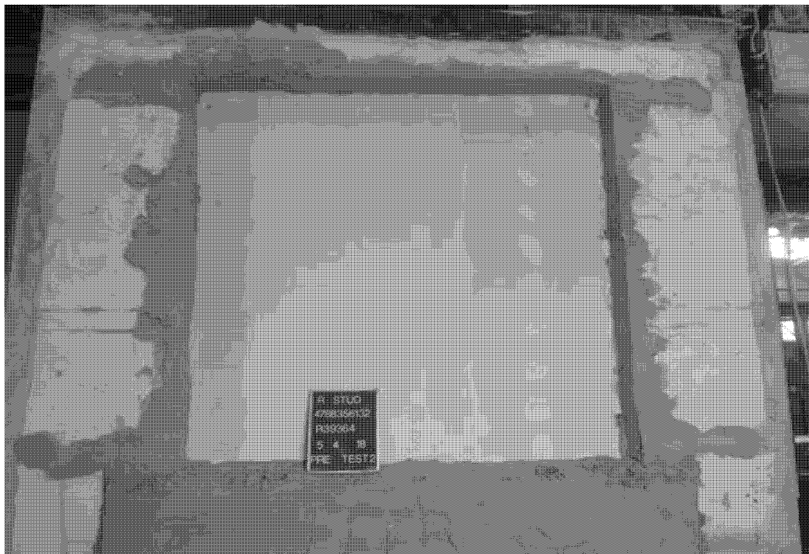
Hose Stream Duplicate – Exposed Face - Pretest
