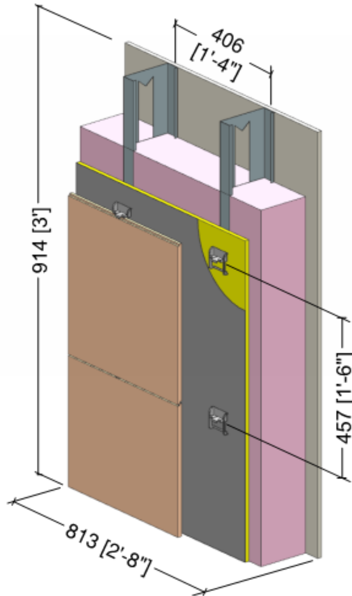
Figure A-1: Exterior View of Modeled Interior Insulated 6" x 1-5/8" Slotted Steel R-Stud Wall Assembly
